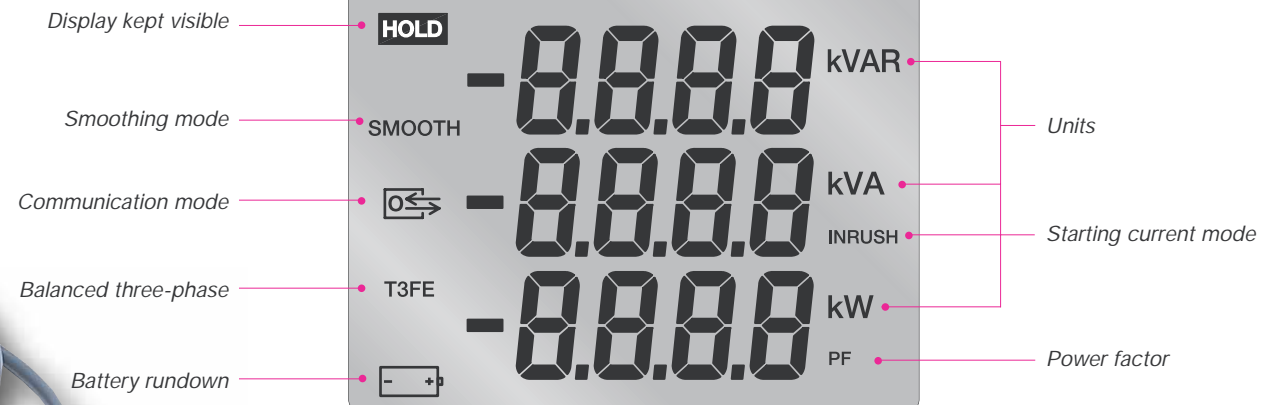
With the 73 x 54.3 mm LCD display, the user knows what the situation is at a glance. The battery rundown indicator light warns him when the period of autonomy is down to one hour.
